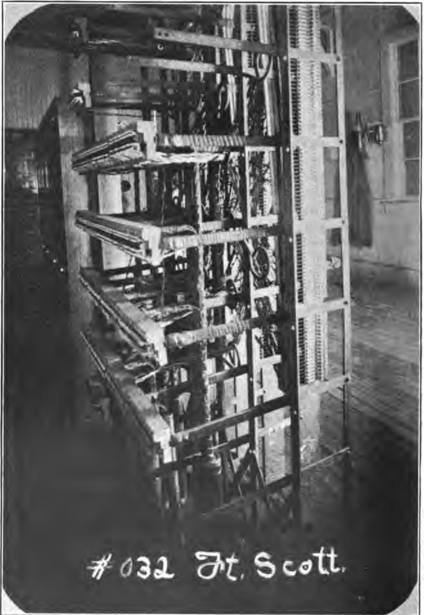
FIG. 94.—Main distributing or cross-connecting frame, Presidio of San Francisco.
